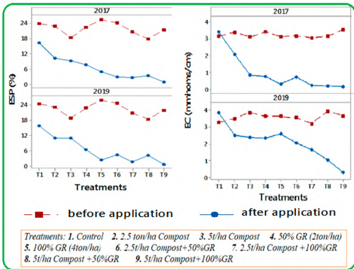
Figure 9. Changing of soil chemical properties status (ECe and ESP) from 2017–2019 after application of gypsum and compost [41].
